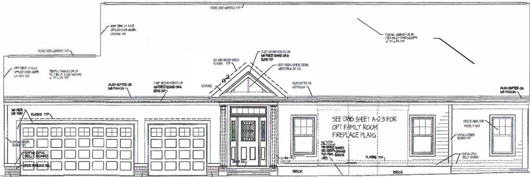
FRONT ELEVATION MODEL F-1300 MODEL F-1301
